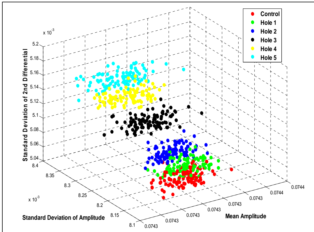
Figure 2: Time/frequency cluster plot for data from specimens with drilled holes
